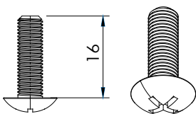
Round head cross screw M6*16
