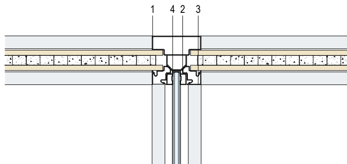
11. T型玻璃-木板-木板屏风 / Glass&wood&wood-T shape
