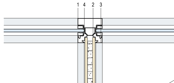
12. T型玻璃-玻璃-木板屏风 / Glass&glass&wood-T shape
